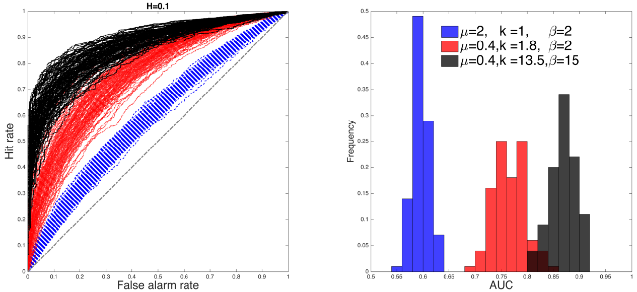
Figure 16: (Left) ROC curve, (Right) the histograms of the AUC for various values.
