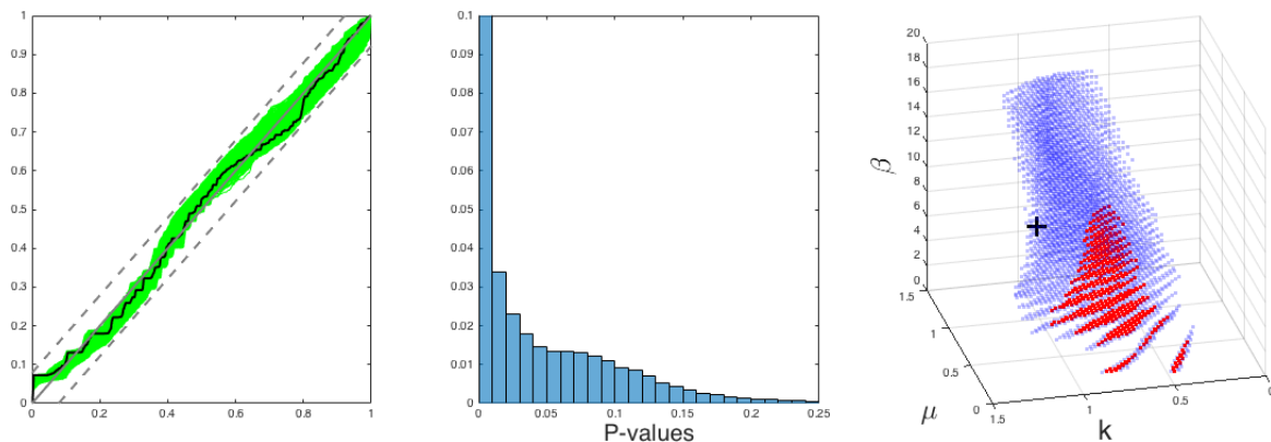
Figure 12: (Left) KS plot of z_k for the Hawkes model. The dash lines indicate the 95% confidence bound and the green curves are the (observed) cumulative distribution obtained from simulated time-series with parameter values with P-values over 0.1. The black curve is the cumulative distribution of a time-series simulated with the MLE. (Middle) A histogram of P-values for uniform parameter grid points (k, \beta, \mu) in [0, 1.5] \times [0, 20] \times [0, 1.5] . (Right) The blue dots shows those parameter with P-value between 0.1 and 0.2 and the red dots shows those with P-value over 0.2. The MLE is shown in the dark + marker.
