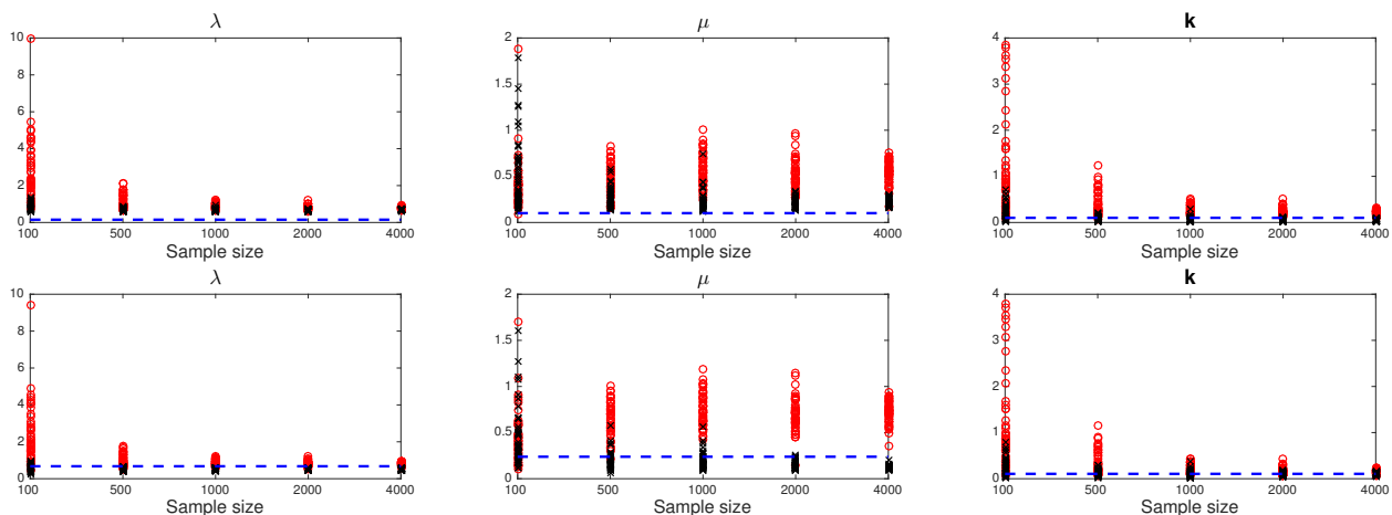
Figure 8: (Top) absolute error |\lambda^*(t) - \lambda(t)| and (Bottom) absolute error |\lambda^o(t) - \lambda(t)| , both of which are averaged over the time t = 40 - 100 for the case \mu = 2 , k = 1.2 and \beta = 2 . The EnPGF results are shown in the black cross mark and the results of a small sample-size PF are shown in red circle. The MLE estimate is plotted with the blue dashed line.
