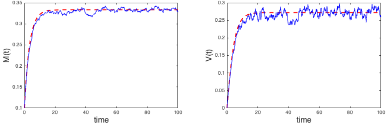
Figure 3: (Solid line) Mean and variance empirically approximated by the sample generated from the Hawkes process (1.1) with parameter values \mu = 0.1, k = 0.7, \beta = 1 . (Dash line) Solutions of the odes (3.2).
