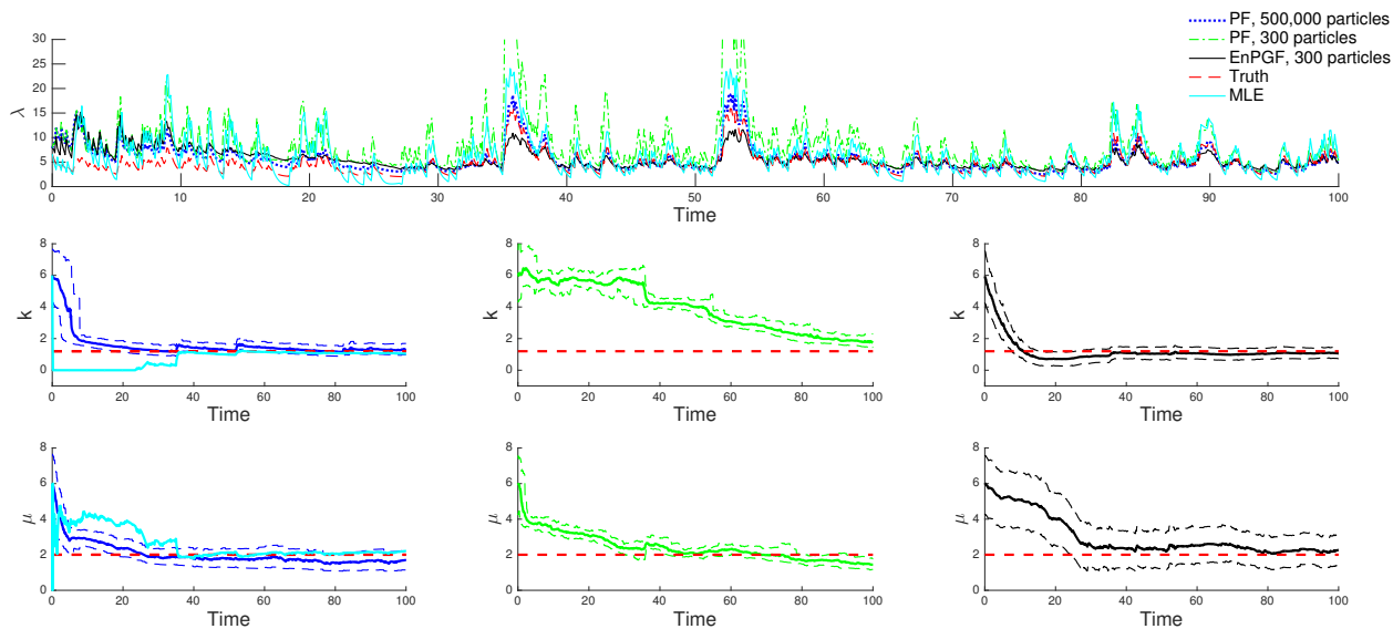
Figure 7: A result for the joint estimation of \lambda , k , and \mu . The sample size for EnPGF and PF is both 300 particles. (Top) Comparison of the sample mean of \lambda(t) . (Middle and Bottom) Comparison of the sample mean and the 90% quantiles of \mu and k for the gold standard (left), PF (middle) and EnPGF (right). Note that the ML estimates for \mu and k is overlaid on the plot of the gold standard result.
