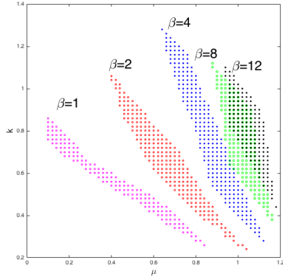
Figure 13: Projection of the parameters with P-value above 0.1 onto the (\mu, k) plane for various values of \beta , see also Figure 12
