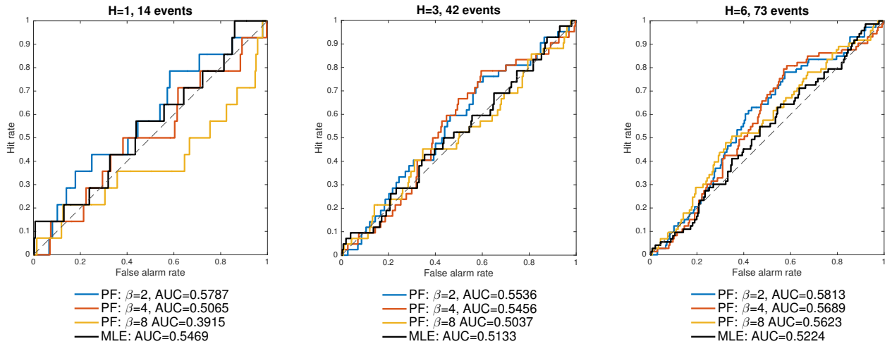
Figure 18: Empirical ROC of PF-based forecast systems for different values of \beta and the Hawkes process with the MLE parameters.
