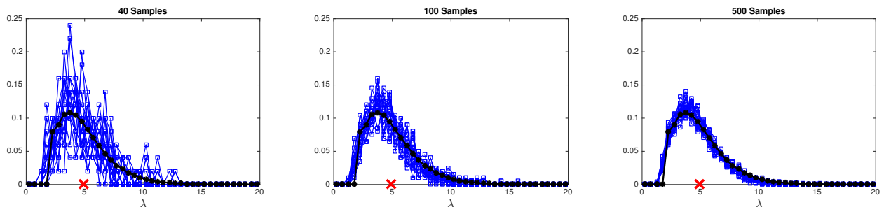
Figure 6: The approximated density of the intensity at t = 100 obtained from the gold standard (black) and EnPGF (blue). The results from 50 experimental runs for EnPGF are plotted for each sample size. The cross mark indicates the true value of the intensity.
