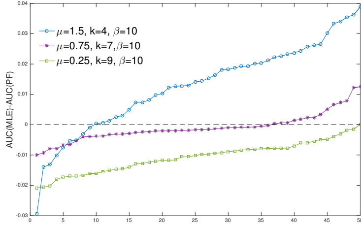
Figure 17: Differences in the empirical AUC obtained from PF-based and MLE-based forecast systems tested for 50 independent experiments. The negative value means the PF-based system results in a higher AUC and vice versa.
