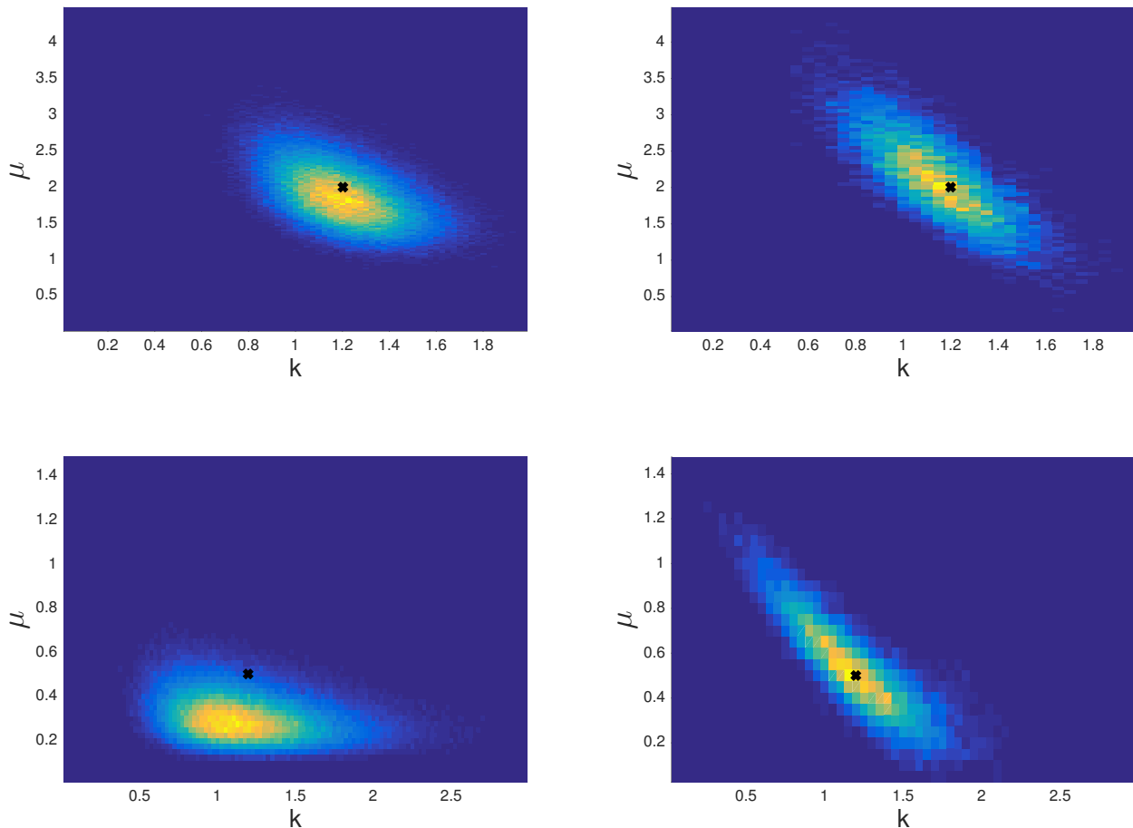
Figure 10: Joint histograms at the final time t = 100 of the gold standard PF (Left) and EnPGF with 5000 sample (Right) for the case \mu = 2, k = 1.2 (Top) and \mu = 0.5, k = 1.2 (Bottom). The cross mark is the true parameter values.
