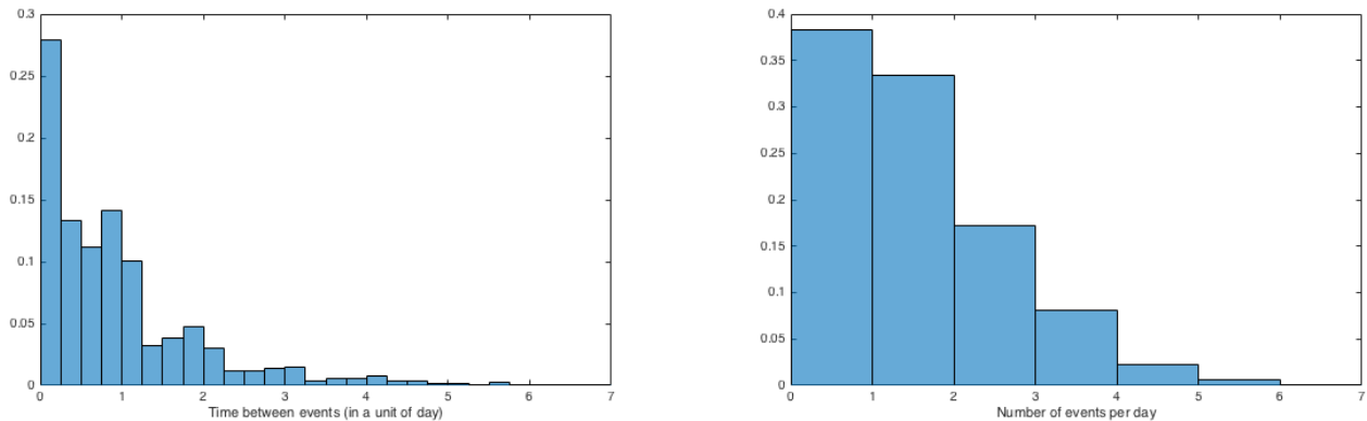
Figure 11: (Left) Histogram of time between two events in a unit of one day. (Right) Histogram of the number of violence crime event per day
