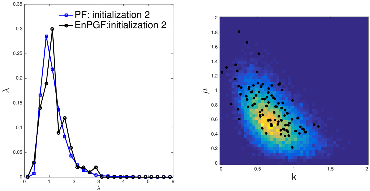
Figure 15: (Left) Comparing the histogram of \lambda for PF (200,000 particles) with EnPGF (100 particles), both of which use the initialization 2. (Right) Empirical joint distribution of k , and \mu at the final step for the gang violence data, which is initialized by using the sample spread obtained from the KS test with the p -values above 0.1. The sample of 100-member EnPGF with the initialization 2 is shown in the solid black dots on top of the approximated density obtained from PF
